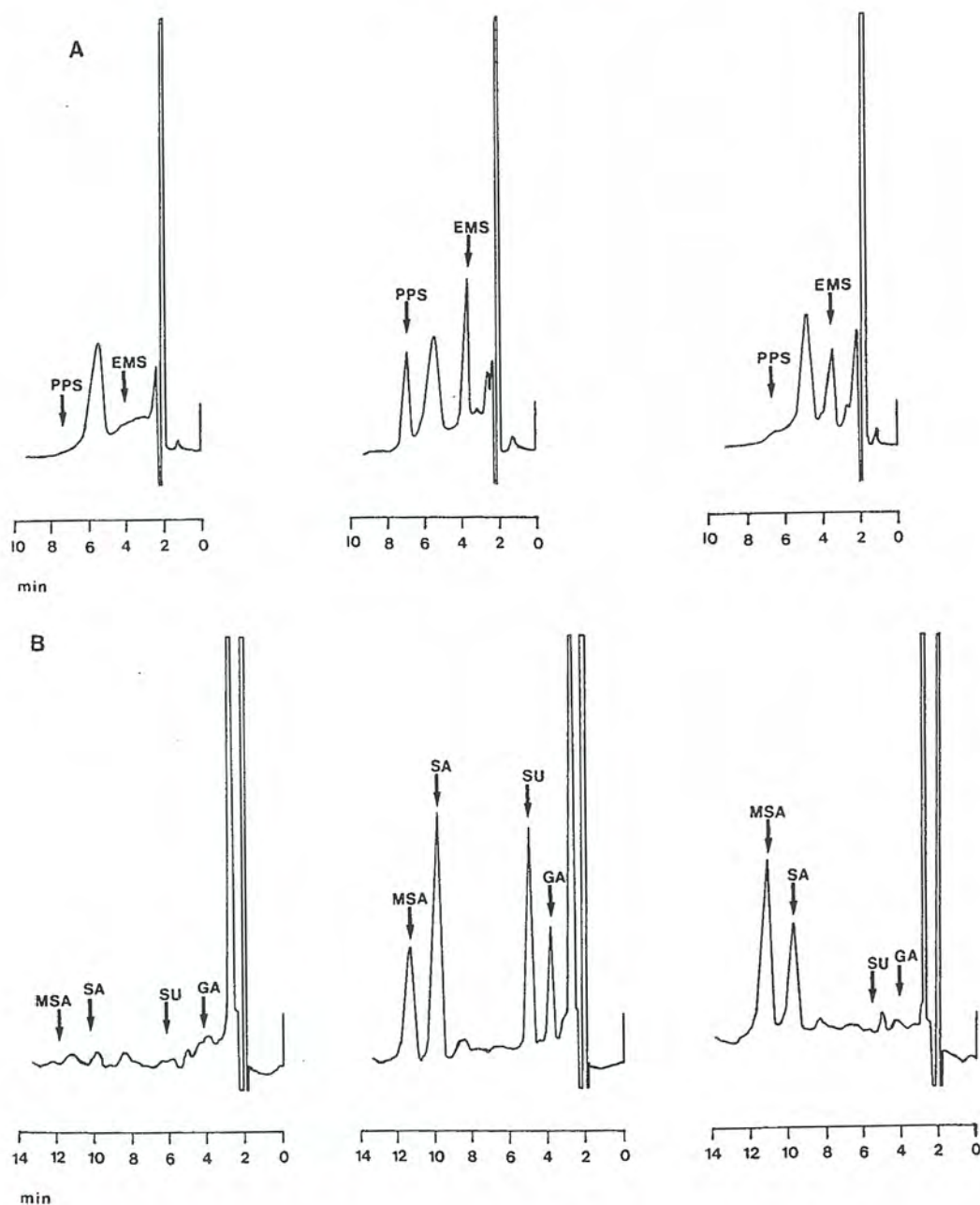
Fig. 1. (A) Chromatograms of extracts from the plasma of one of the volunteers (subject B.W.). Left: Pre-topical dose; middle: drug-free plasma spiked with 1 \mu\text{g/ml} EMS and PPS; right: 6 h post topical dose. (B) Chromatograms of extracts from the plasma of one of the volunteers (subject B.W.). Left: Pre-topical dose; middle: drug-free plasma spiked with 0.5 \mu\text{g/ml} of each of the metabolites; right: 6 h post topical dose.
